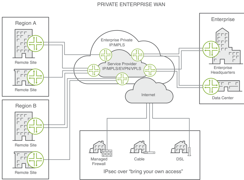
Figure 5: Private enterprise WAN is almost entirely managed by the enterprise. Remote sites and home users are brought into the network using IPsec over public transport
