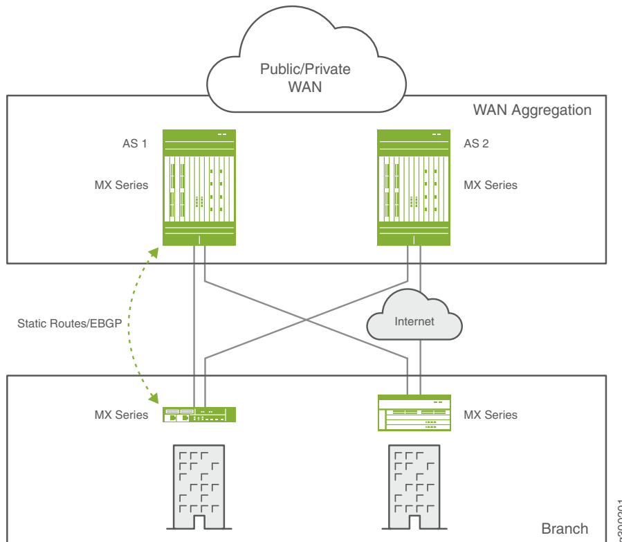
Figure 6: Sample WAN aggregation routers that combine multiple remote branch sites into a single enterprise WAN
