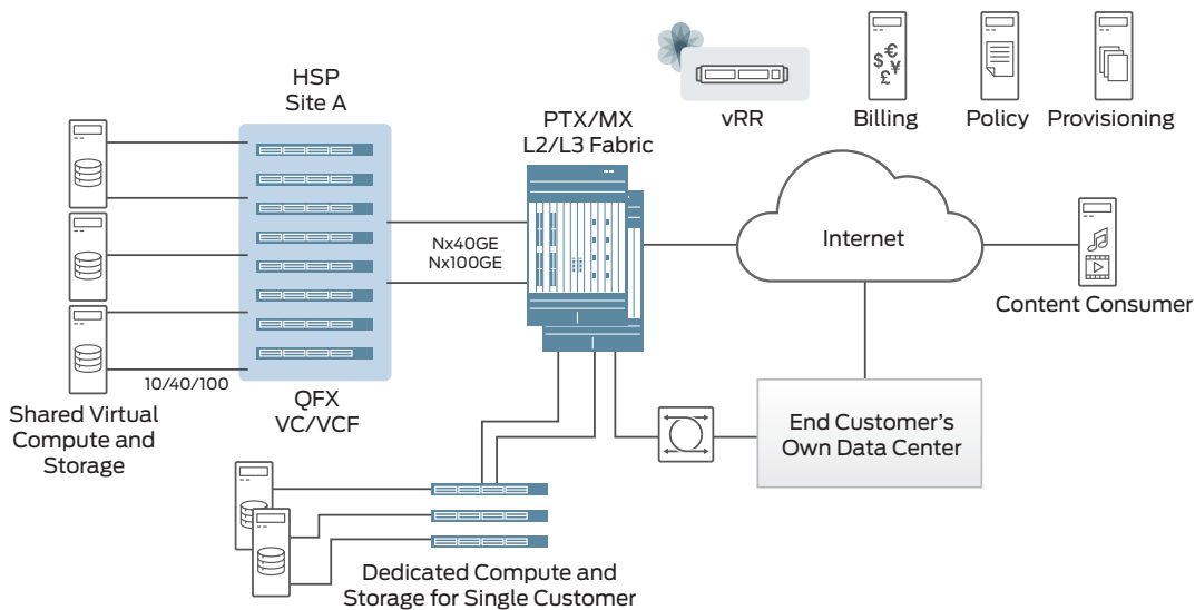
Figure 3: Reference architecture for Juniper-based managed private/hybrid cloud services solution
